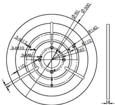
Turntable plate ECO S300
